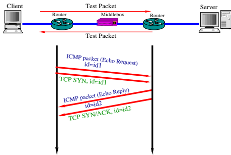
(a) Client initiated TCP SYN-SYN/ACK Handshake
