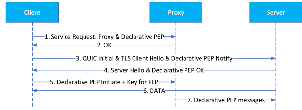
Figure 2: Declarative PEP negotiation/key exchange
